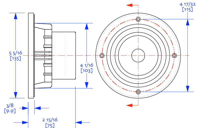
D: 2 magnets / bezel cover
