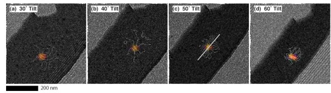
FIG. 3. (Color online) The equiphasic contour lines of the out-of-plane component of a vortex in a notched permalloy nanowire are shown for different tilt angles of the sample [(a) 30^\circ , (b) 40^\circ , (c) 50^\circ , and (d) 60^\circ ].
