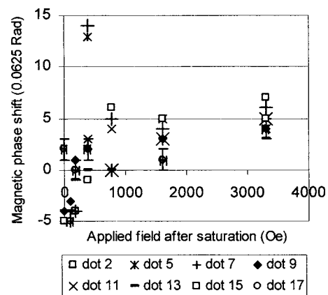
FIG. 7. In-plane magnetic phase shifts across individual dots, measured in a direction perpendicular to the applied field. Dot numbers refer to Fig. 4 inset.
