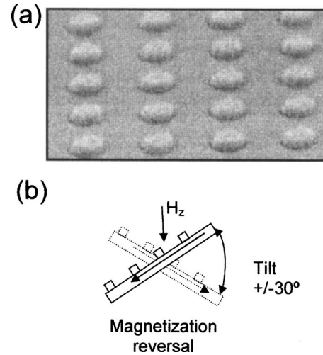
FIG. 1. (a) Scanning electron microscope image of nominally 100-nm diameter and 20-nm-thick Co dots fabricated on Si in a square array of side 200 nm. (b) Schematic diagram showing the experimental setup for applying an external magnetic field. H_z is the applied field direction, which is parallel to the electron microscope optic axis.
