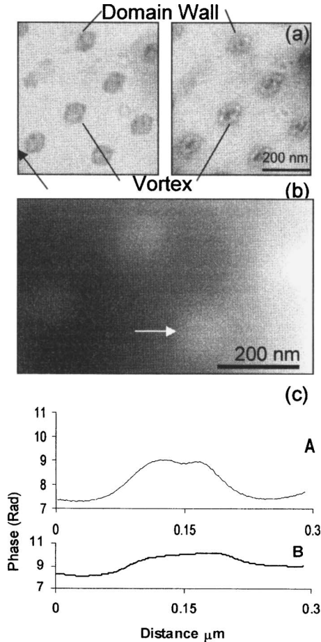
FIG. 9. (a) Fresnel defocus images acquired at \pm 108\text{-}\mu\text{m} defocus. The arrow indicates the applied field direction. (b) Phase image [bottom 4 dots from (a)] obtained by applying the transport of intensity equation to the Fresnel TEM images. (c) Corresponding line profiles indicating the phase changes across the dot indicated with the white arrow in (b), both parallel (A) and perpendicular (B) to the applied field direction.
