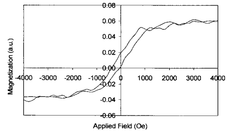
FIG. 6. In-plane hysteresis loop for \sim 6 \times 10^{10} dots measured using VSM.
