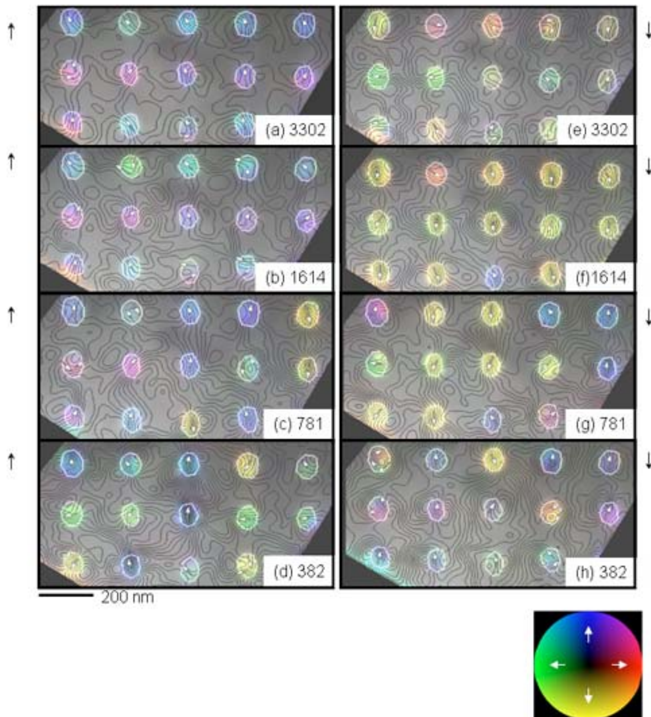
FIG. 3. (Color online) Magnetic induction maps showing remanent states in the square array of Co dots measured using electron holography. The spacing between adjacent contours is 0.0625 rad. The applied fields in oersted are shown, with \uparrow and \downarrow indicating the directions of the indicated applied in-plane field after saturation in the opposite direction. The color wheel indicates the direction of magnetization by the color and the intensity represents the strength of the magnetic signal.
