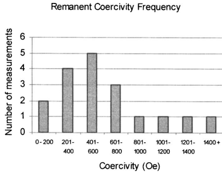
FIG. 8. Frequency plot of the coercivity values of individual dots. The mean value of the coercivity is 670 \pm 403 Oe. The large standard deviation results from the spread in the magnetic properties of the dots, and not from the experimental error.
