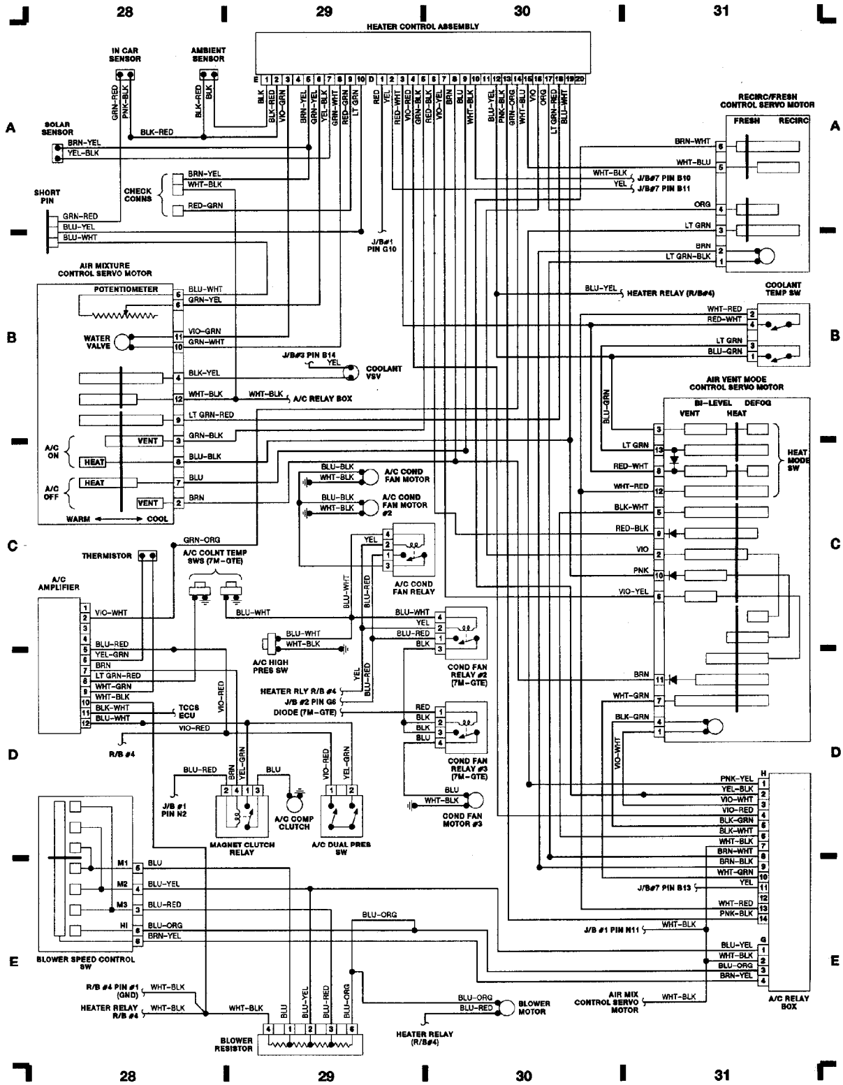
90G07368 Fig. 8: A/C & Heating
