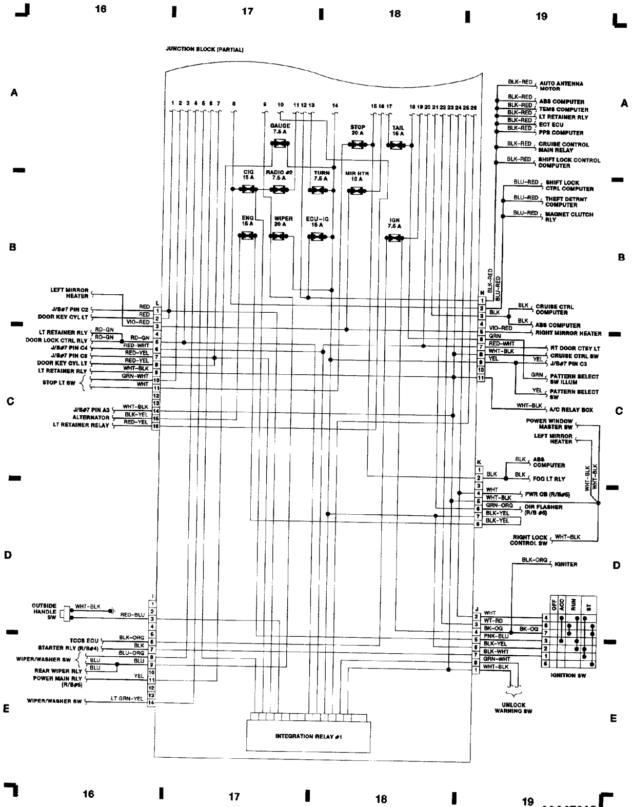
Fig. 5: Fuse Block No. 1 (2 of 2)
