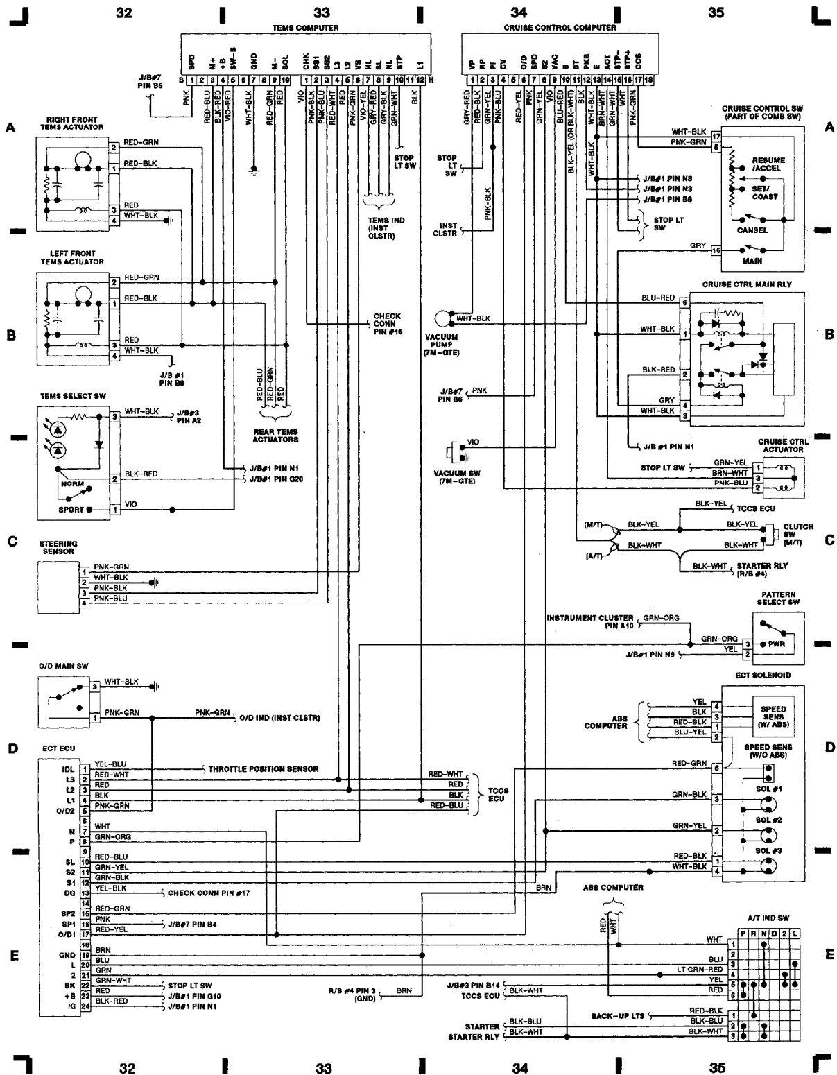
Fig. 9: Suspension Control, Automatic Transmission Control and Cruise Control
