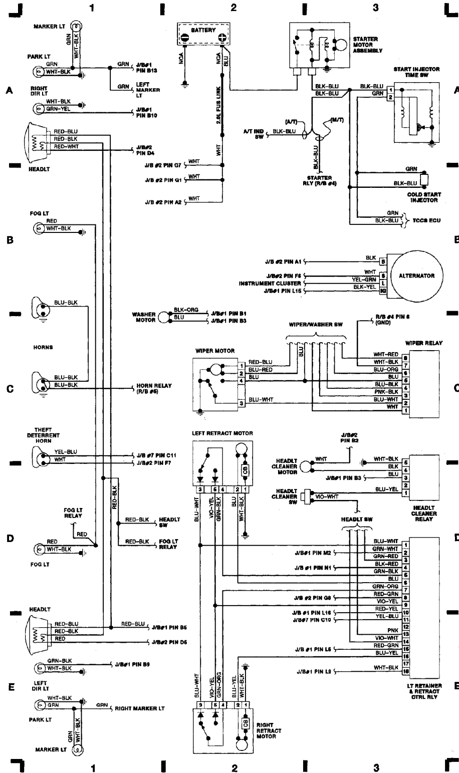
90B07361 Fig. 1: Engine Compartment & Headlights
