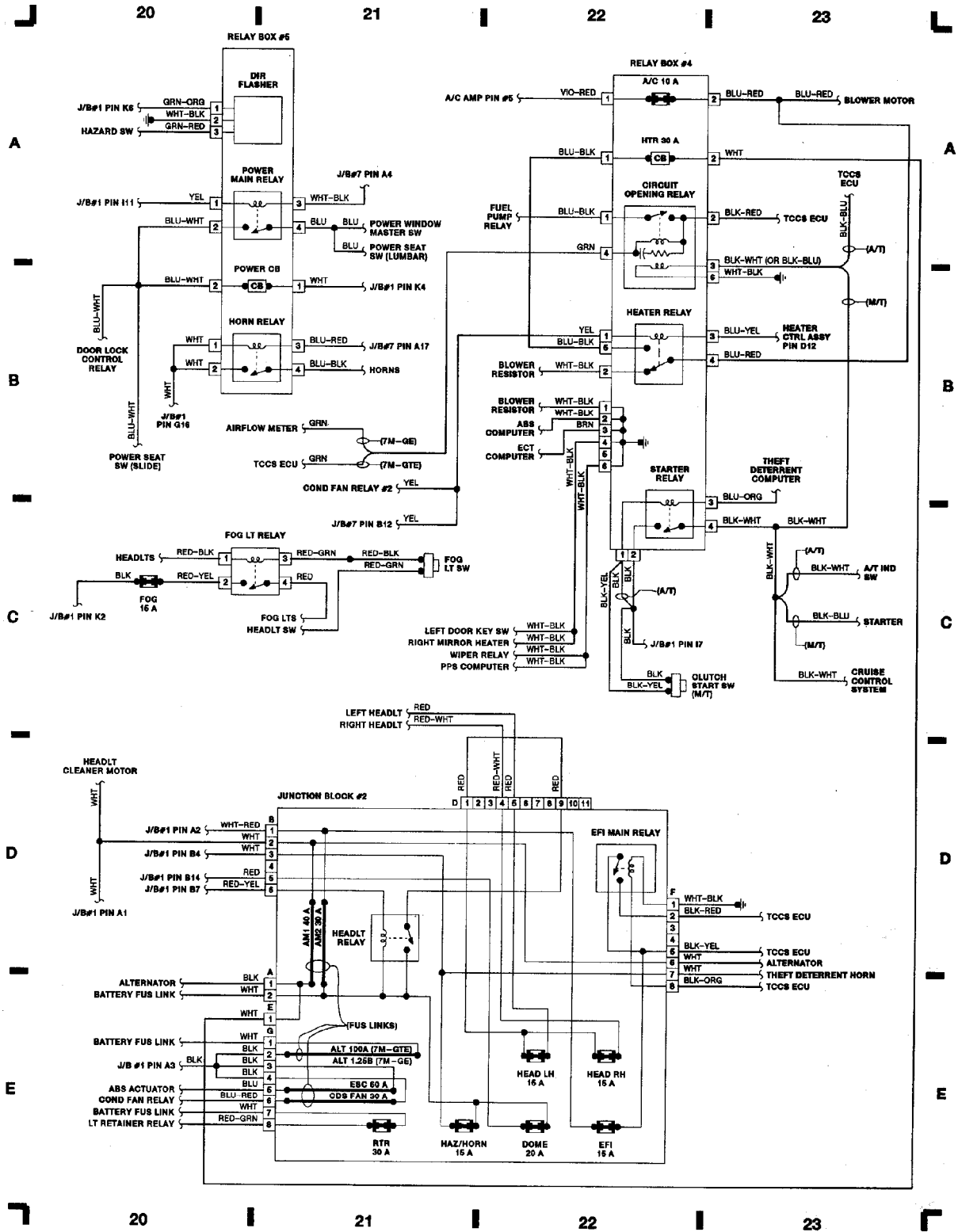
90C07366 Fig. 6: Relays & Headlight Control
