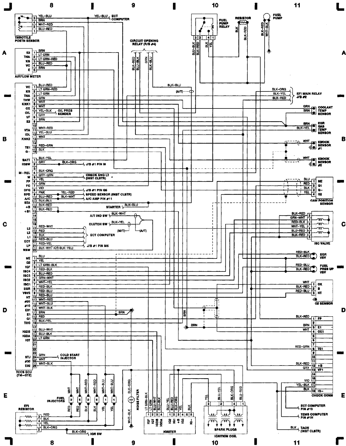
90F07363 Fig. 3: Computer Engine Control (Turbo)
