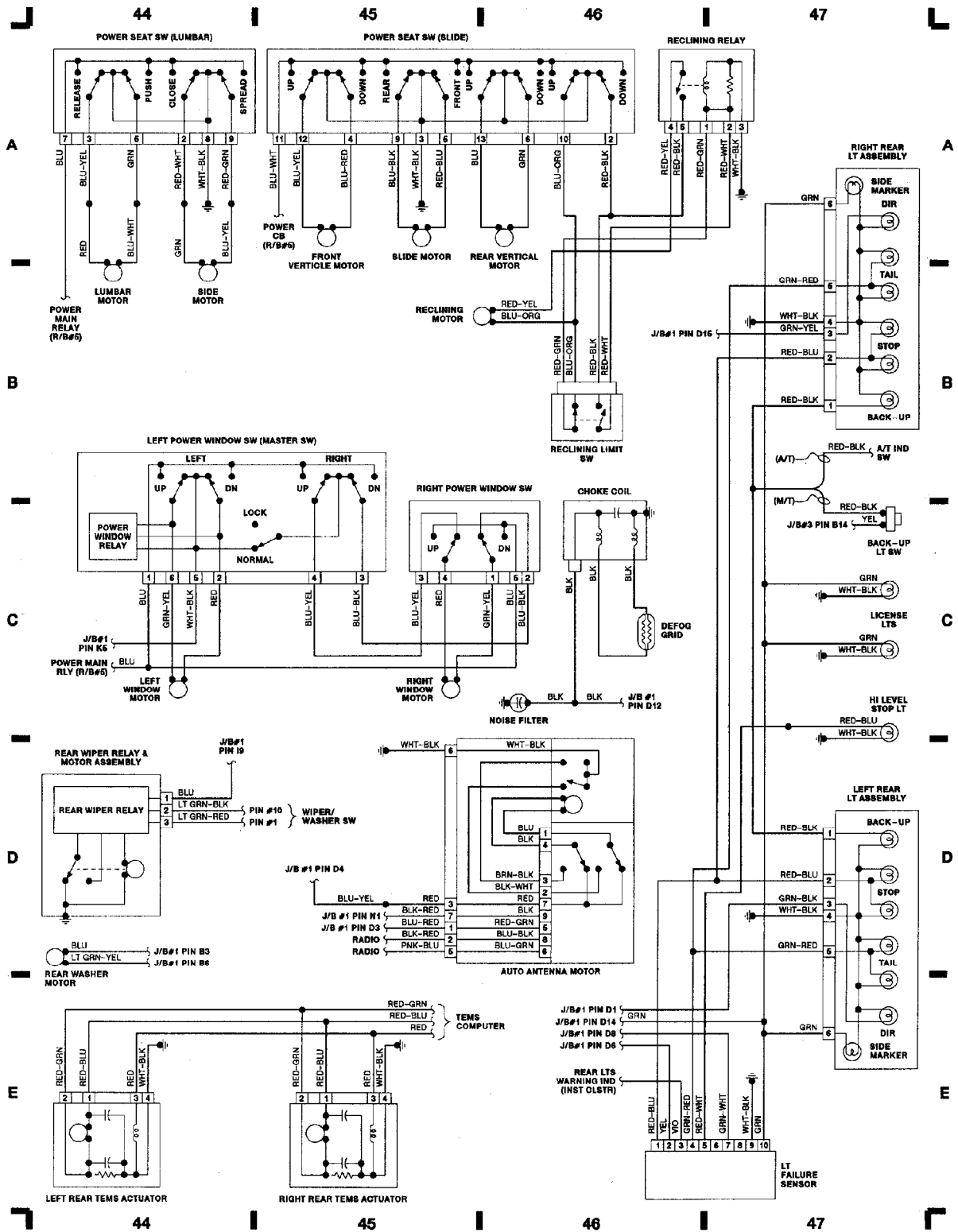
90E07372 Fig. 12: Passenger Compartment & Taillights
