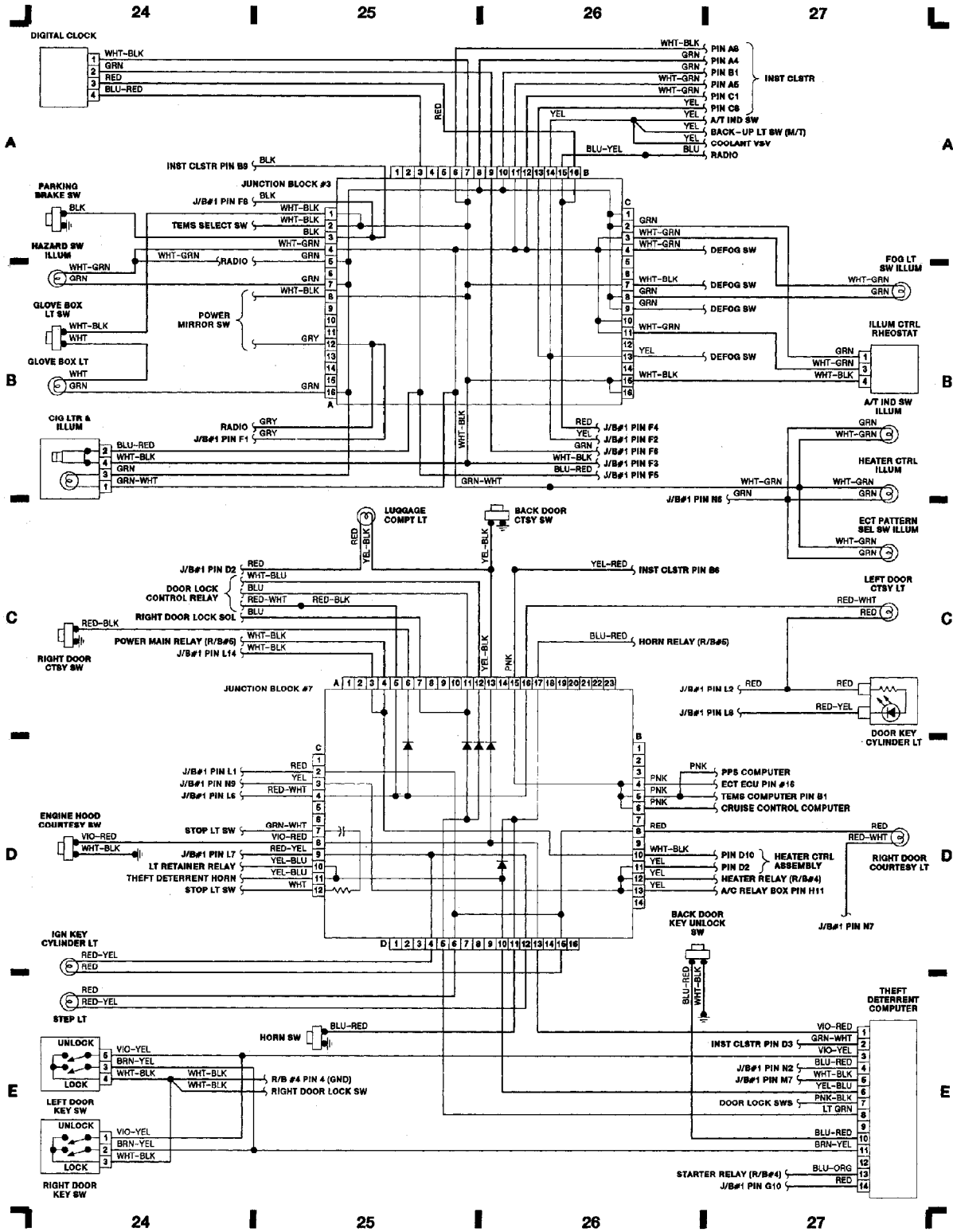
90E07367 Fig. 7: Fuse Blocks No. 3 and No. 7
