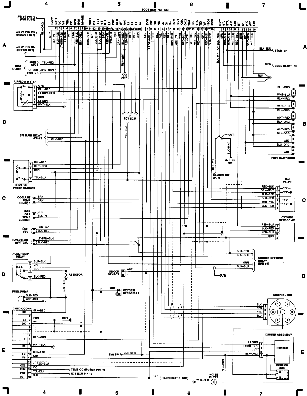
90D07362 Fig. 2: Computer Engine Control (Non-Turbo)
