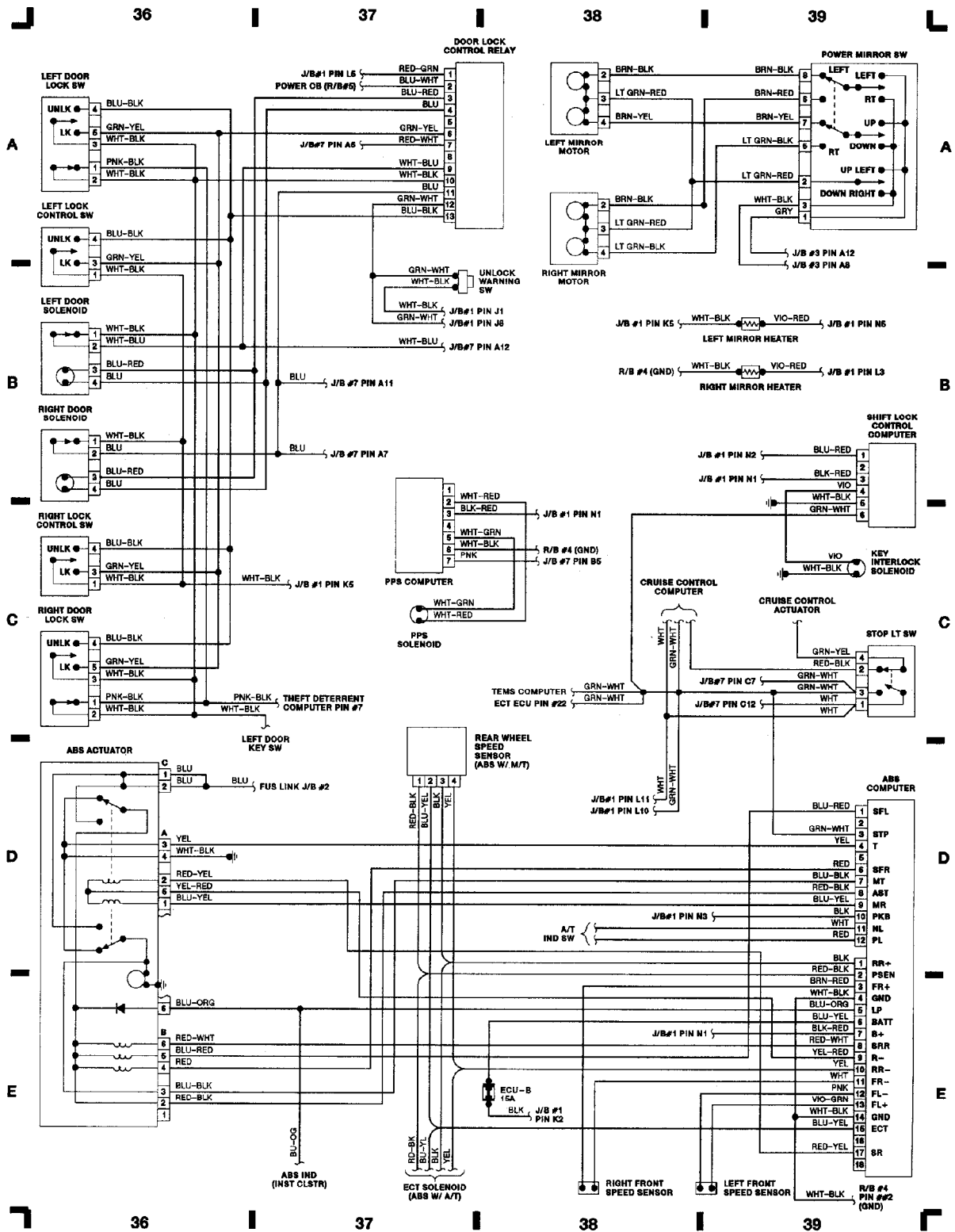
90A07370 Fig. 10: Power Doors, Power Mirrors and Anti-Lock Brake System
