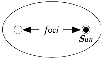
Kepler's First Law: Ellipses
