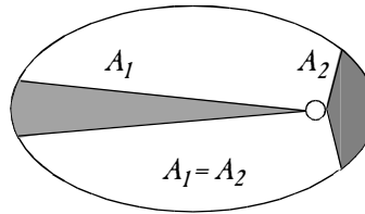
Kepler's Second Law: Equal Areas
