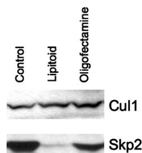
Fig. 4 Lipitoid-mediated siRNA transfection is compared to siRNA transfection with a standard transfection reagent. Skp2 siRNA2 (100 nM) was used with lipitoid or Oligofectamine as the transfection reagent. LacZ siRNA (100 nM) was used as a control. T98G cells were lysed 48 h after transfection followed by Western Blot analysis with specific antibodies against skp2 and the loading control cul1, respectively. The faint skp2 band in the lipitoid treated cells as compared to the relatively intense skp2 band in the Oligofectamine treated cells demonstrates the efficiency of lipitoid for gene silencing in complex with this siRNA.
