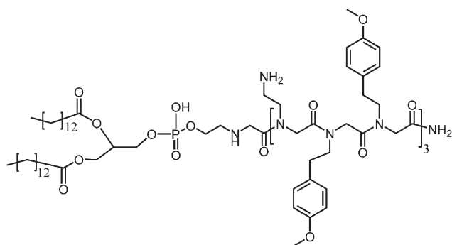
Fig. 1 Chemical structure of the lipitoid transfection reagent DMPE-(NaeNmpeNmpe) 3 consisting of a phospholipid conjugated to a cationic peptoid backbone (DMPE, dimyristoyl phosphatidyl-ethanolamine; Nae, N -(2-aminoethyl)glycine; Nmpe, N - p -methoxyphenethylglycine).
