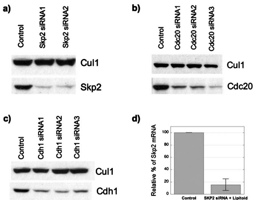
Fig. 3 Transfection of siRNA leads to effective downregulation of target proteins through RNA interference. Transfection experiments were carried out in T98G cells using three different protein targets. A variety of siRNA sequences (50 nM) for each target protein were tested individually. Transfections were carried out with the lipitoid DMPE-(NaeNmpeNmpe) 3 as the transfection reagent and LacZ siRNA as negative control. Targeted protein levels were determined 48 h after transfection. Western Blot analyses with specific antibodies against the targeted proteins and the loading control cul1 show effective downregulation of the target proteins (a) skp2, (b) cdc20 and (c) cdh1. (d) Skp2 mRNA levels in T98G cells treated with 50 nM skp2 siRNA and lipitoid were evaluated by extracting whole RNA from treated cells 48 h after transfection, followed by real-time RT-PCR with specific primers for Skp2. The extent of Skp2 mRNA expression is plotted relative to the control (LacZ) siRNA treated cells. All mRNA was normalized to GAPDH amounts.
