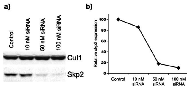
Fig. 2 Lipitoid transfects siRNA and causes concentration dependent downregulation of the targeted protein. Varying concentrations (10 nM–100 nM) of skp2 siRNA2 were tested in T98G cells. Transfection experiments were done with the lipitoid DMPE-(NaeNmpeNmpe) 3 as transfection agent and LacZ siRNA as the control siRNA (50 nM). (a) Western Blot analysis with specific antibodies against skp2 and the loading control cull1 was performed 48 h after transfection. (b) Skp2 amounts as quantified from the Western Blot.
