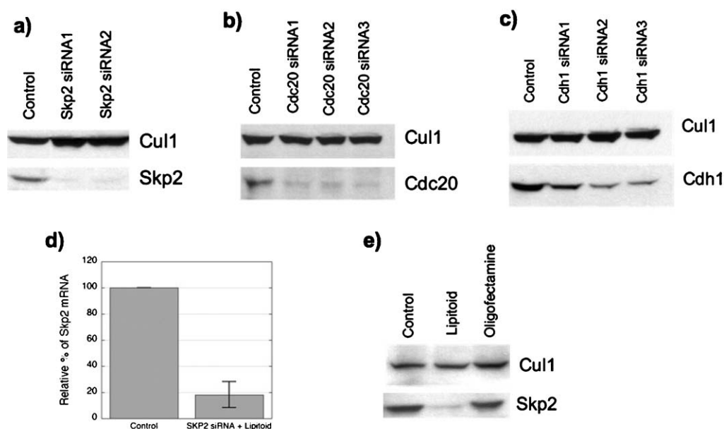
Fig. 5 Lipitoid is capable of delivering siRNA into IMR-90 primary cells. Western Blot analyses show efficient downregulation of the targeted proteins (a) skp2 , (b) cdc20 , and (c) cdh1 , respectively. In all experiments, siRNA (50 nM) was transfected into IMR-90 primary cells using the lipidoid DMPE-(NaeNmpeNmpe) 3 as a transfection reagent and LacZ siRNA (50 nM) as negative control. (d) The decrease in Skp2 mRNA levels in IMR-90 upon transfection with skp2 siRNA with lipidoid as quantified by real-time RT-PCR, confirm RNA interference effect. (e) The Western Blot demonstrates that the lipidoid transfection of skp2 siRNA was efficient and resulted in significant decrease of skp2 expression, while skp2 siRNA with Oligofectamine does not generate any quantifiable difference in the expressed skp2 amount in this cell line.
