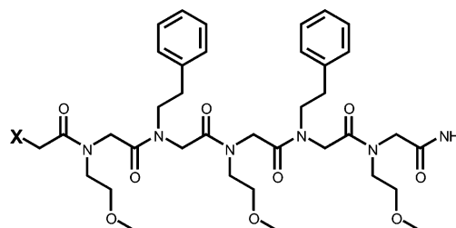
Figure 2. Model peptoid pentamer. X denotes chemoselective functionality.
