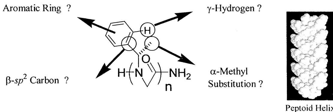
Figure 1. Monomer structural elements of the peptoid helix. Each of these elements were investigated by the systematic synthesis of analogs.
