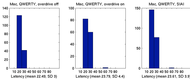
Figure 9: Histograms of latency of QWERTY keyboard to audio out latency for Max/MSP 4.3 under MacOS 10.2.8 on an unloaded machine with 64-sample IO and signal buffers and various scheduling modes.
