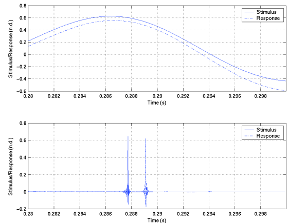
Figure 3: Plots of stimulus and response impulses band-limited to 100 Hz (upper plot) and 22050 Hz (lower plot). The test configuration and procedure is identical to that of Figure 2. The increase in latency from the 100 Hz case to the 22050 Hz case is readily apparent.
