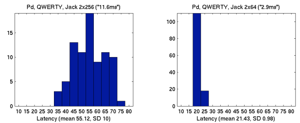
Figure 11: Histograms of latency of QWERTY keyboard to audio out latency for Pd under Linux (configured as described in section 3), using Jack. The left histogram is for Jack using 256-sample buffers; the right is for 64-sample buffers.
