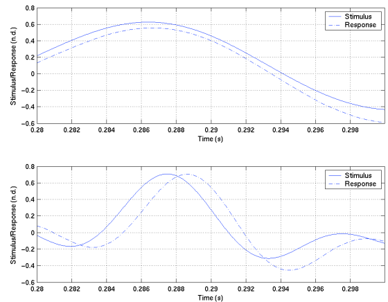
Figure 2: Plots of stimulus and response impulses band-limited to 100 Hz (upper plot) and 125 Hz (lower plot). (Linux PC using an M-Audio Omni I/O, HW through)
