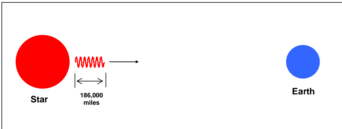
Figure 1. A star emits a one-second pulse of light toward the Earth ( c assumed constant).
