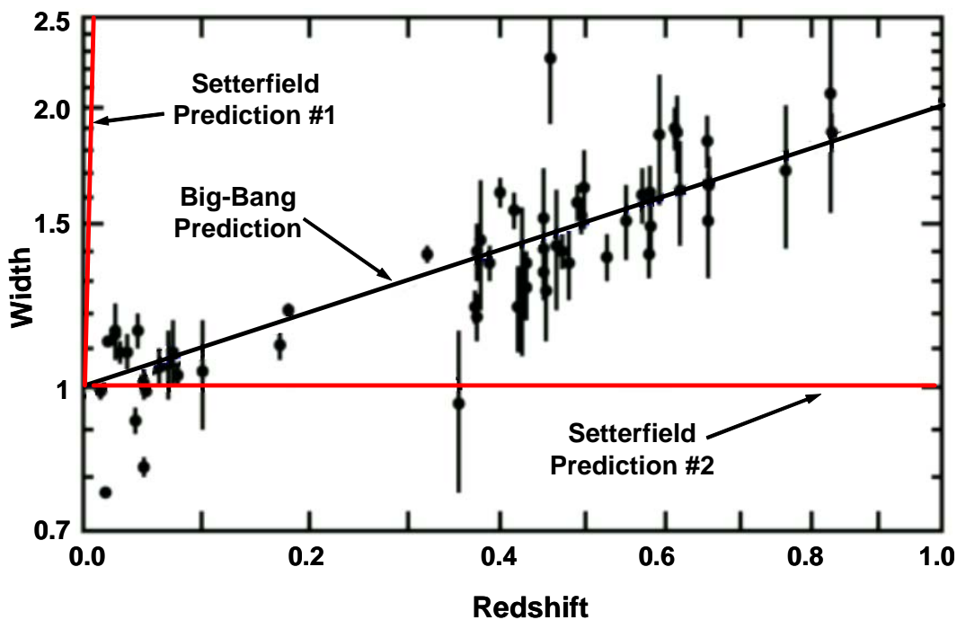
Figure 17. Supernova light curve width vs. distance. 90
