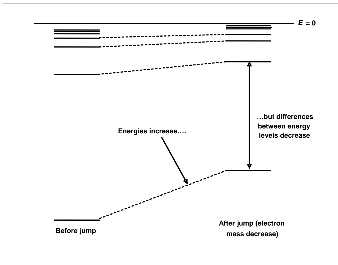
Figure 21. Atomic energy levels before and after speculated “quantum jump.”
