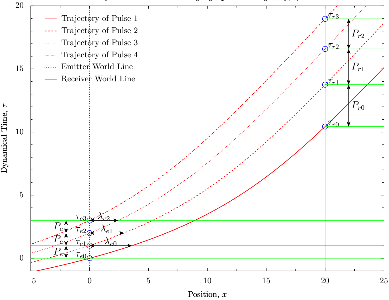
Photon Trajectories with a Changing Speed of Light, \zeta(\tau) = 1 + 3e^{-0.3\tau}
