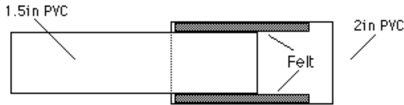
Fig. 8: Giving the Drawtube a Good Fit
