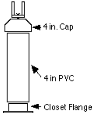
Fig 16: Exploded View of Short Pier Mount
