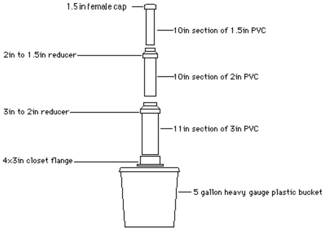
Fig. 13: Bucket Mount plans and parts
