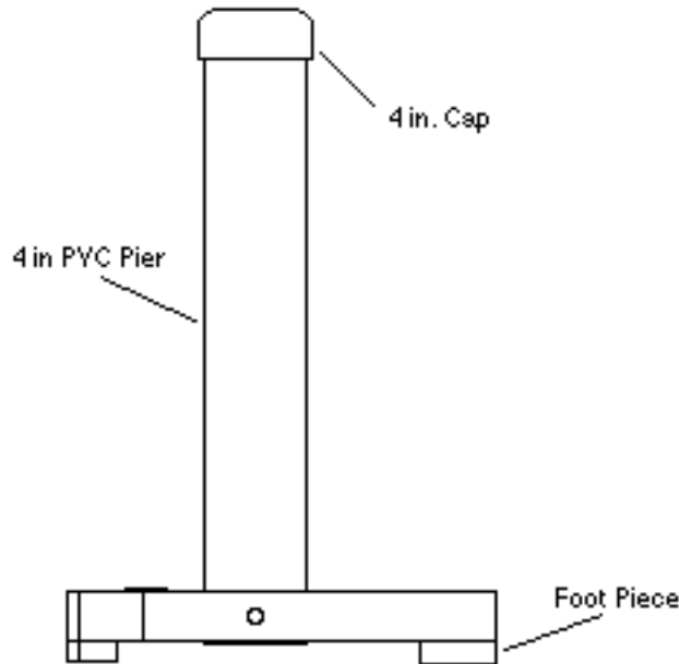
Fig. 15: Completed Pier Mount
