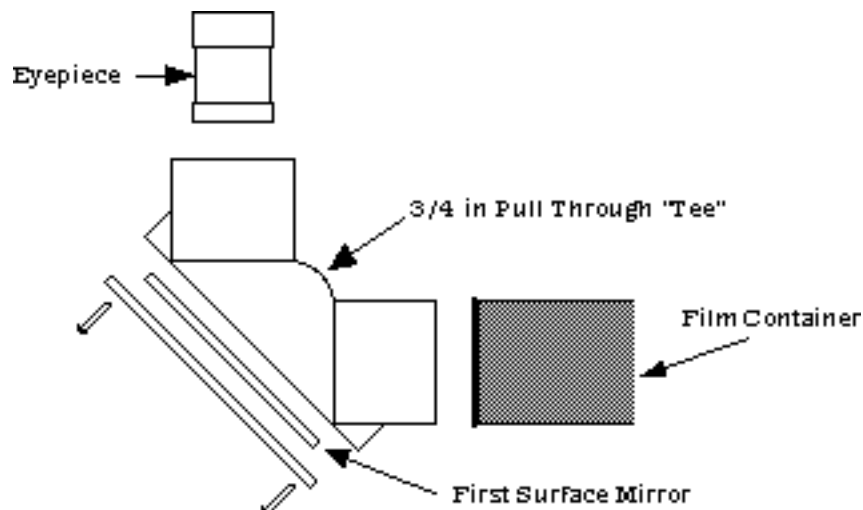
Fig. 2: Making a Diagonal
