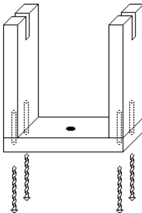
Fig. 11: Assembling the fork
