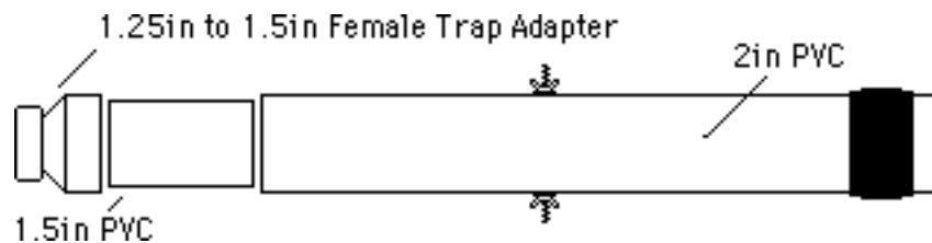
Fig. 9: Exploded View of the PVC Telescope
