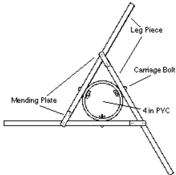
Fig. 14: Pier legs as seen from below
